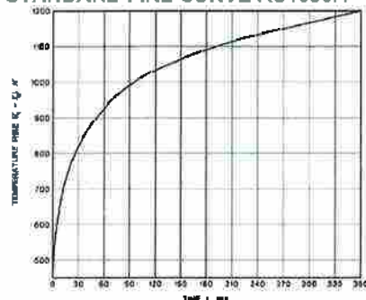
FIGURE 2.3 STANDARD FIRE CURVE AS1530.4
