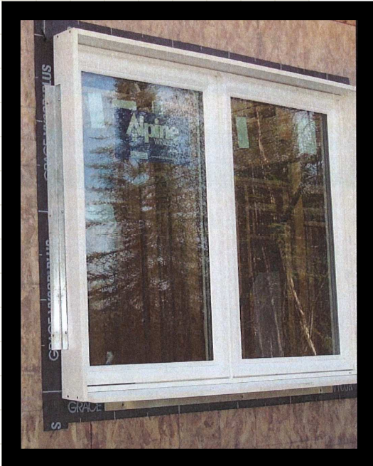
Figure 12. Alternate Window Box Mount Courtesy: Cold Climate Housing Research Center
